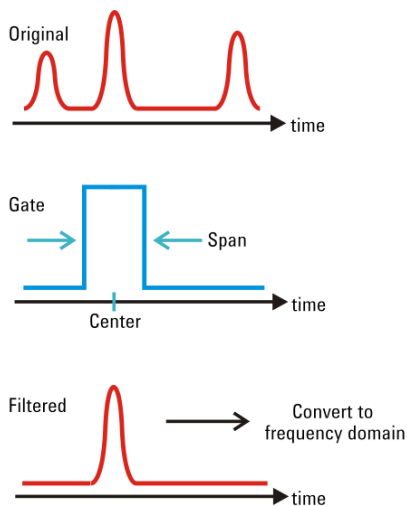
Figure 6. Simplified example of an ideal time domain response having three peaks and the results when a time “gate” is applied to the original response
