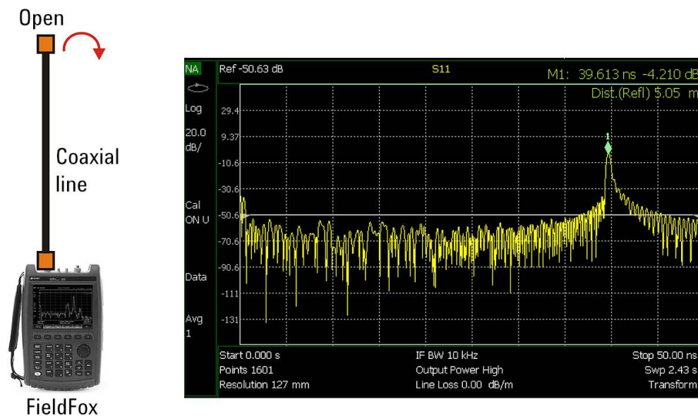
Figure 8. Test configuration and time domain response of a short length of RG58 coaxial cable terminated in an open
