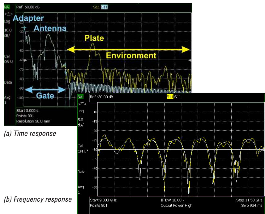
Figure 7. (7a) time and (7b) frequency domain responses of the X-band antenna system with and without a gate function applied to the measured data
