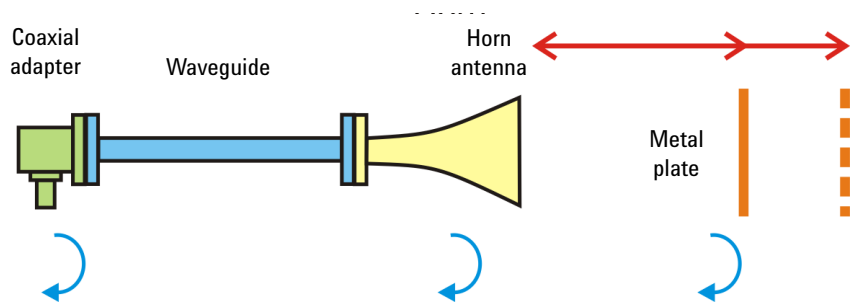
Figure 3. Configuration for measuring the frequency domain and time domain responses of an over-the-air measurement using an X-band horn antenna
