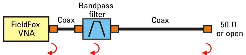
Figure 9. Test configuration for a system that includes two coaxial cables interconnected with a bandpass filter and terminated in either an open or a 50-ohm load
